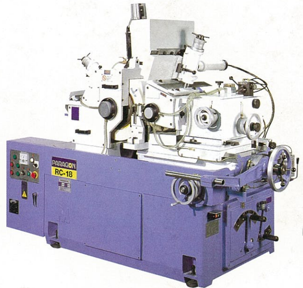
CENTERLESS GRINDING MACHINE
